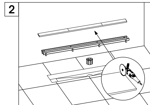
2. Cut the tile insert to fit the tray.
