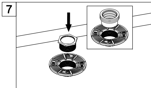
7. Connect the adapter and install on the flange (Hexagonal thread adapter and rubber adapter are optional).
