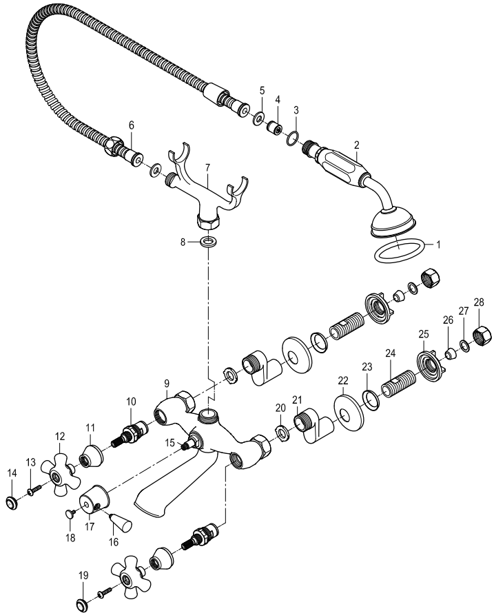
Cold Handle: KSH266PXC
