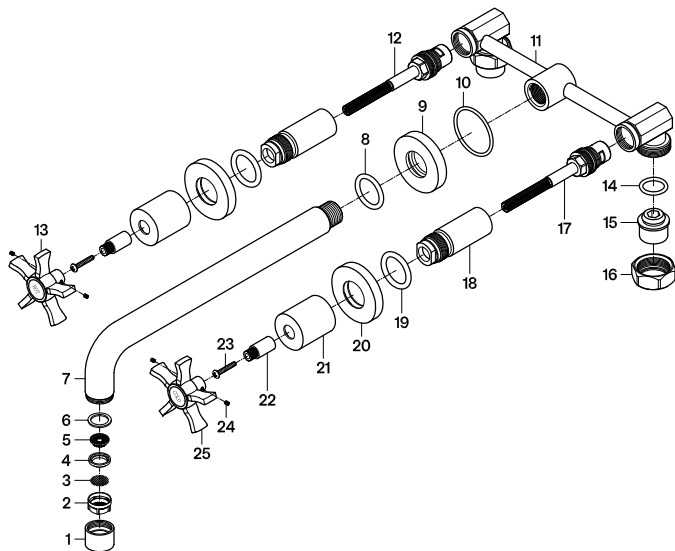
Hot Cartridge: No.12- KSRPL8000C
