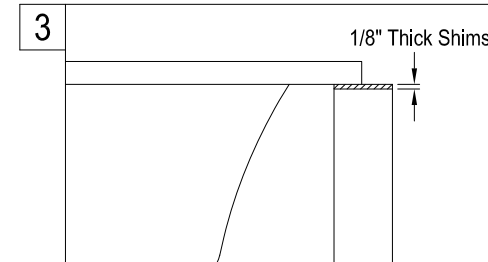
3. Make sure to leave an access area to be able to make the plumbing and drain connections once the tub is in place. Place 1/8" thick shims on top of the finished deck around the perimeter where the tub rim will make contact with the deck.
