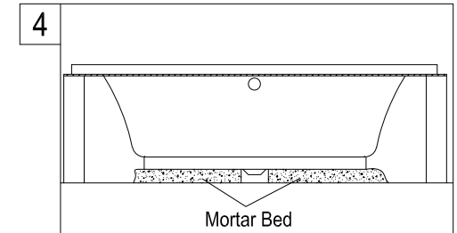
4. Pour a mortar bed under the area where the tub will be resting, except on the area around the drain, the mortar bed should be thick enough to provide ample support to the tub.
