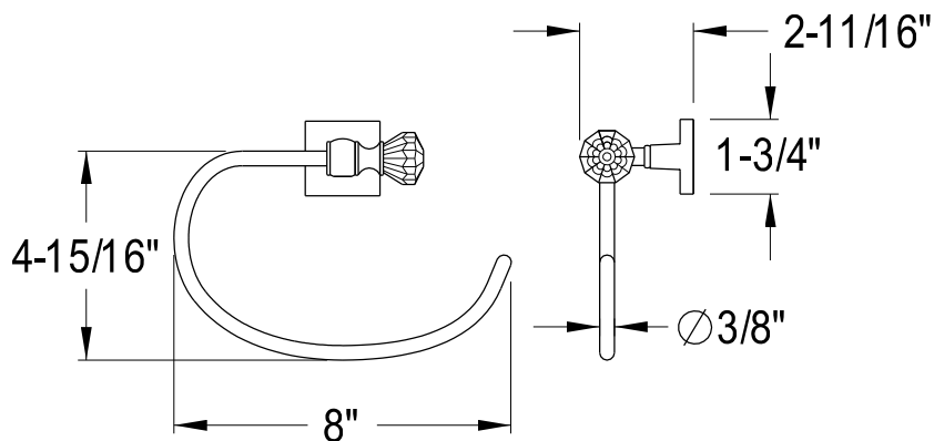
Towel Ring
