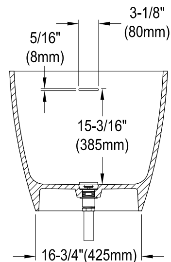
Section B-B
