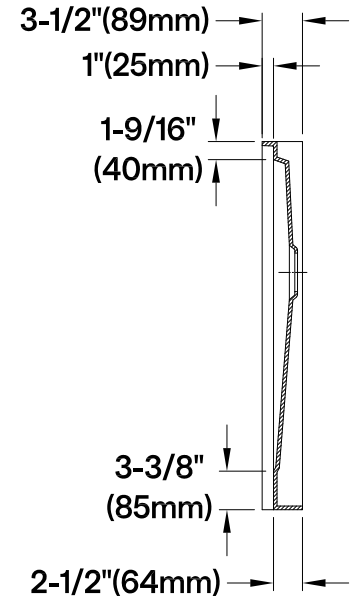
Section B-B
